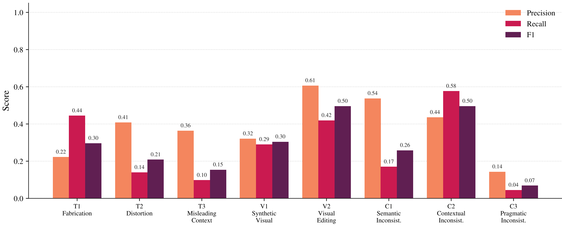
qwen3_5_4b: 8-way Distortion Taxonomy Per-label P/R/F1
