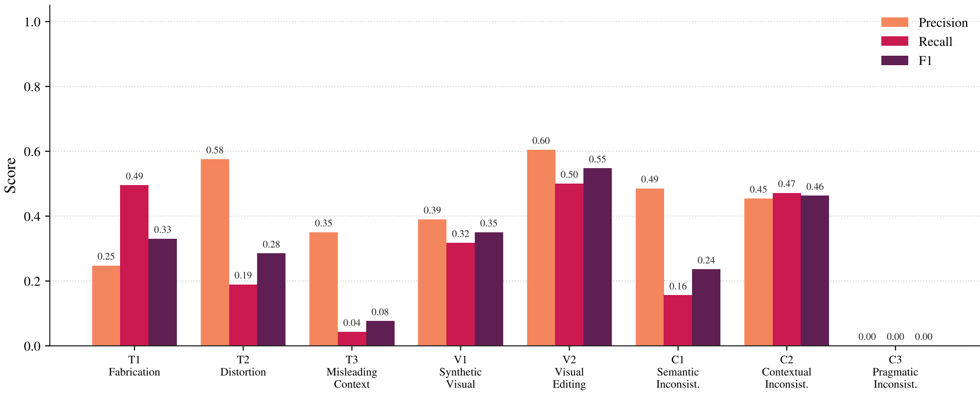
qwen3_5_9b: 8-way Distortion Taxonomy Per-label P/R/F1
