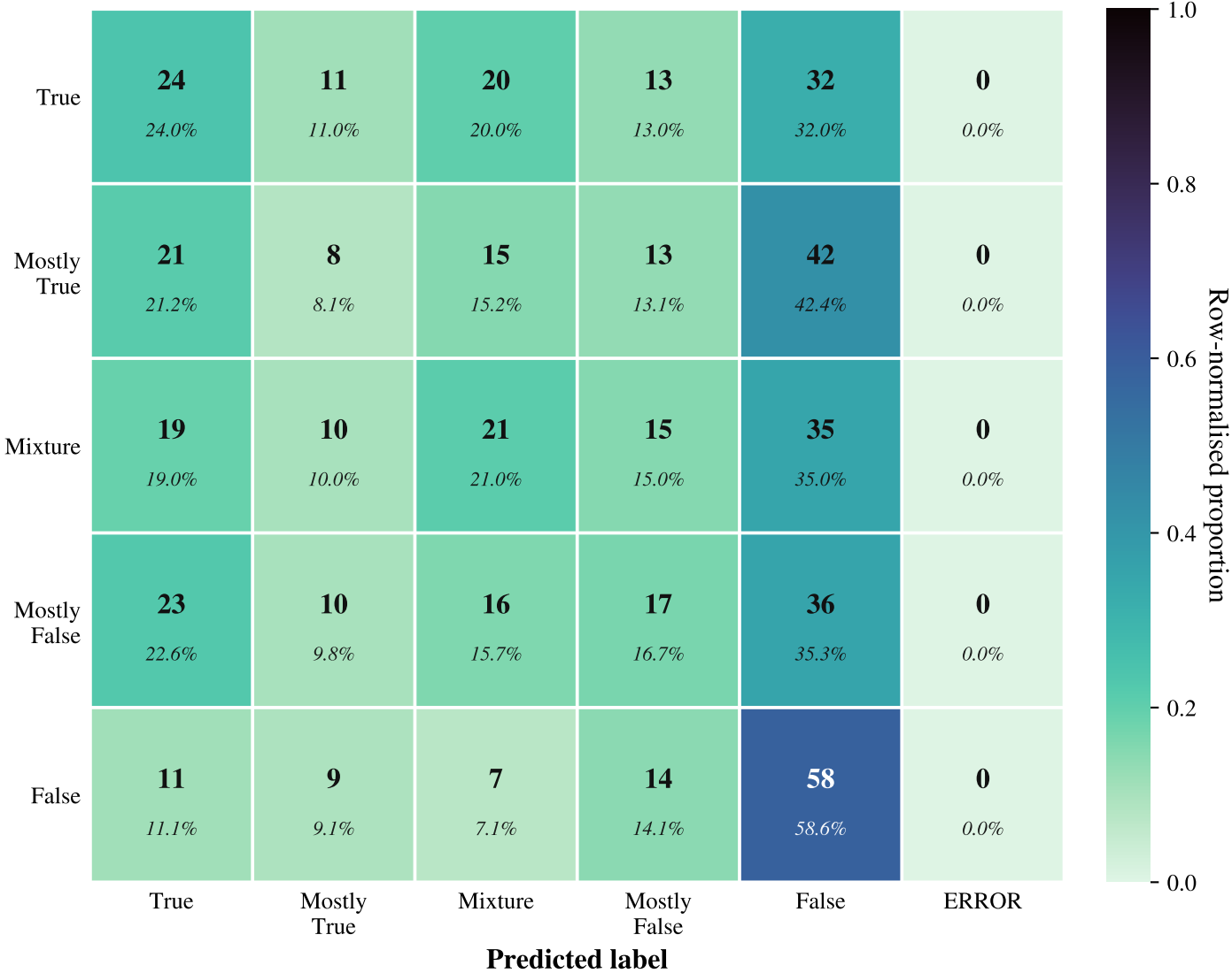
qwen3_5_9b: 5-way Verdict Confusion Matrix
