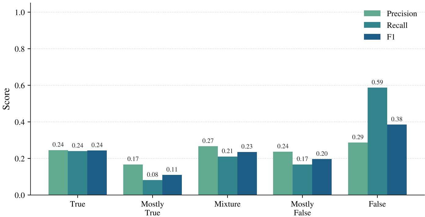
qwen3_5_9b: 5-way Verdict Per-class P/R/F1
