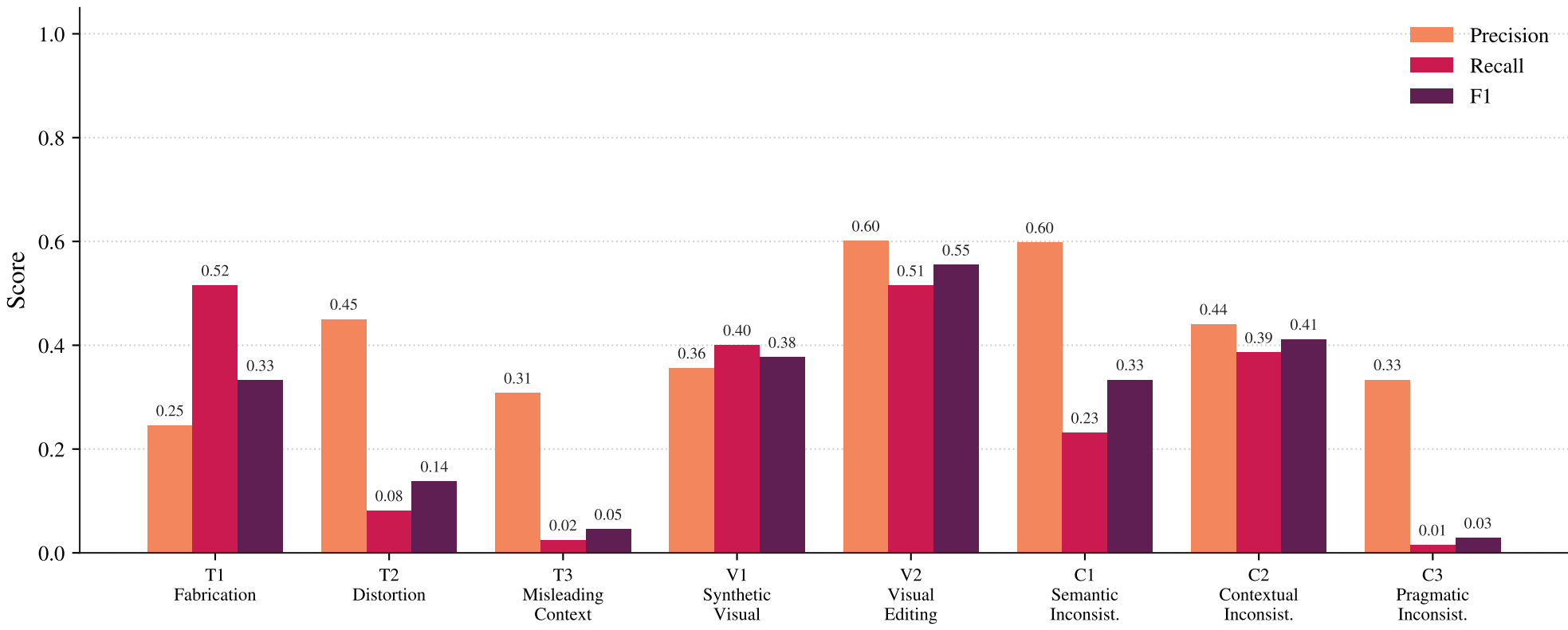
qwen3_6_27b: 8-way Distortion Taxonomy Per-label P/R/F1
