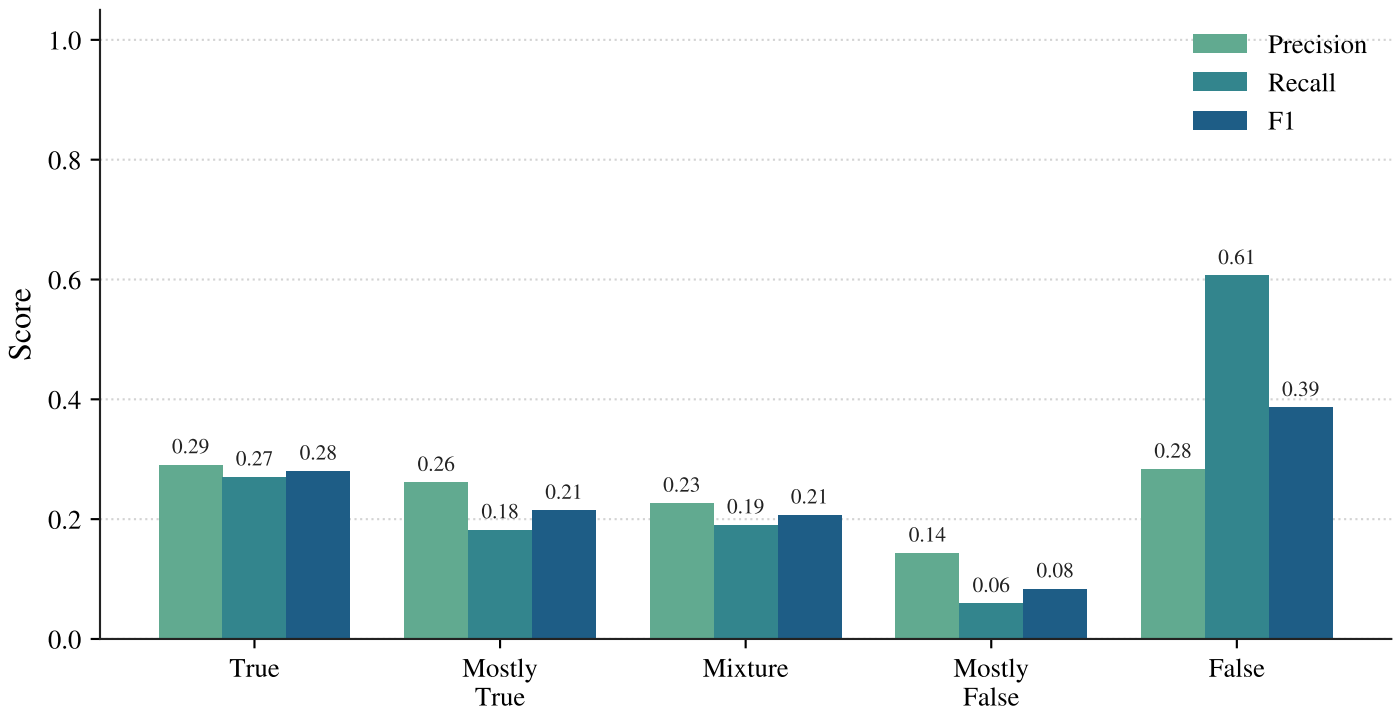
qwen3_6_27b: 5-way Verdict Per-class P/R/F1
