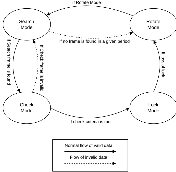
Figure C.2: State machine diagram for the single-branch asynchronous flywheel algorithm.
