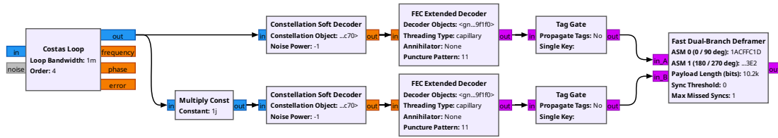
Figure 4.4: Dual-branch receiver architecture with parallel Viterbi decoding and fast synchronization.
