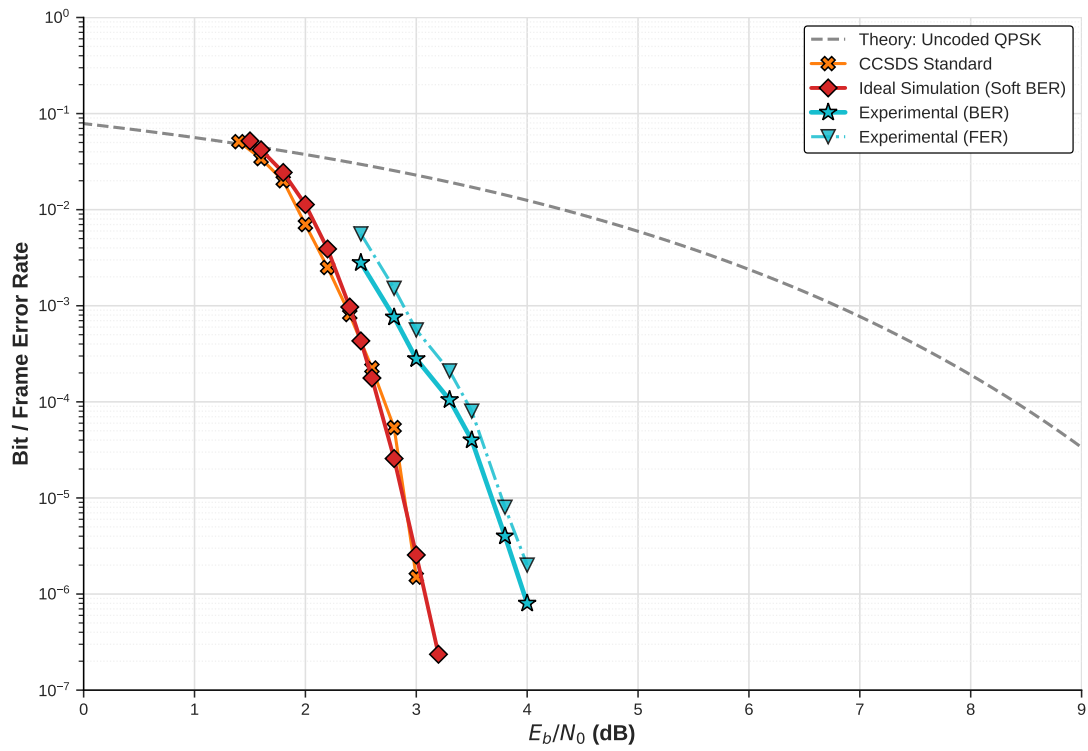
Figure 5.3: Final bit and frame error rate performance of the complete SDR pipeline. The experimental curve illustrates the real-time execution including Doppler tracking and dual-branch synchronization, compared against the ideal simulated soft-decoding performance, the theoretical CCSDS limit, and the uncoded QPSK baseline.
