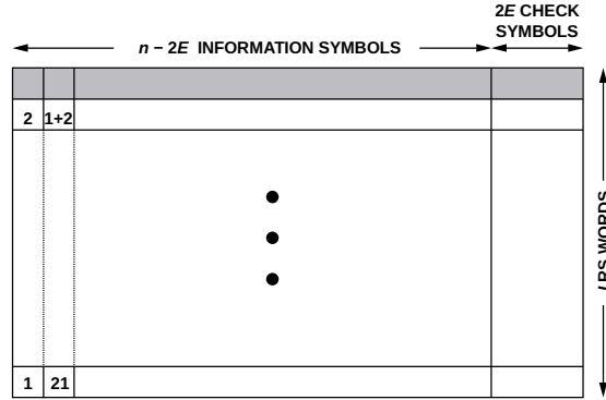
Figure 1.8: Rectangular block interleaver matrix of depth I . A contiguous channel error burst of length B symbols is distributed upon de-interleaving such that no single codeword absorbs more than \lceil B/I \rceil errors. You can find an example in Figure B.2 → p. 36 .
