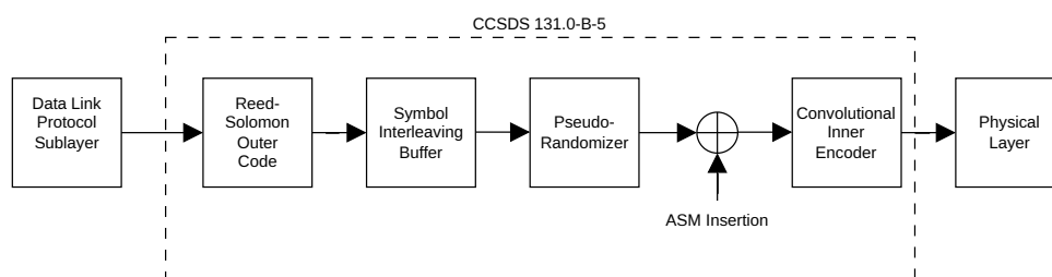
Figure 1.1: Block diagram of the transmitter.
