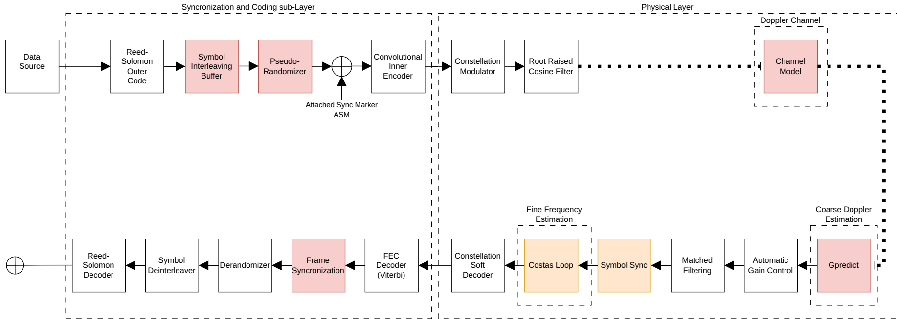
Figure B.1: Complete block diagram of the end-to-end communication system implemented in GNU Radio. Red blocks represent custom DSP modules developed specifically for this project and orange blocks indicate existing library modules that were modified.
