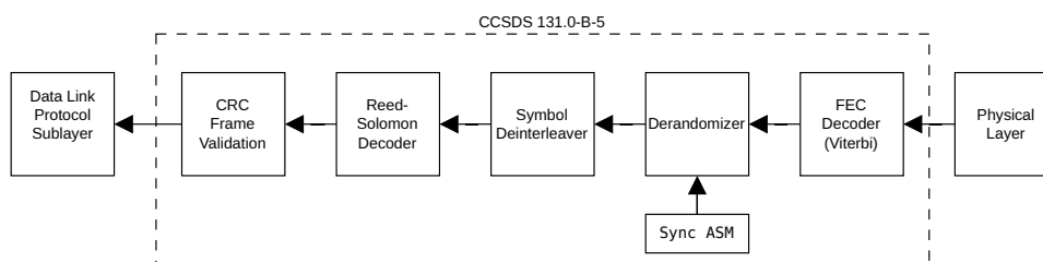
Figure 1.2: Block diagram of the receiver.
