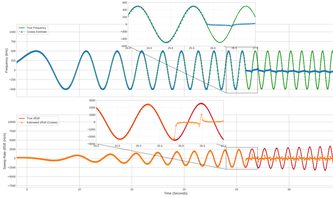
Figure 3.16: Frequency tracking performance: True vs. Estimated frequency. The Costas Loop loses lock at a sweep rate of 2.5 kHz/s for a simulated loop bandwidth of B_n = 5 mrad/s.
