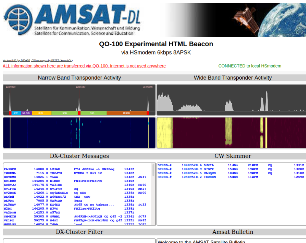
Figure 6.3: Demodulated HTML dashboard extracted from the QO-100 multimedia beacon, displaying live telemetry and transponder status.
