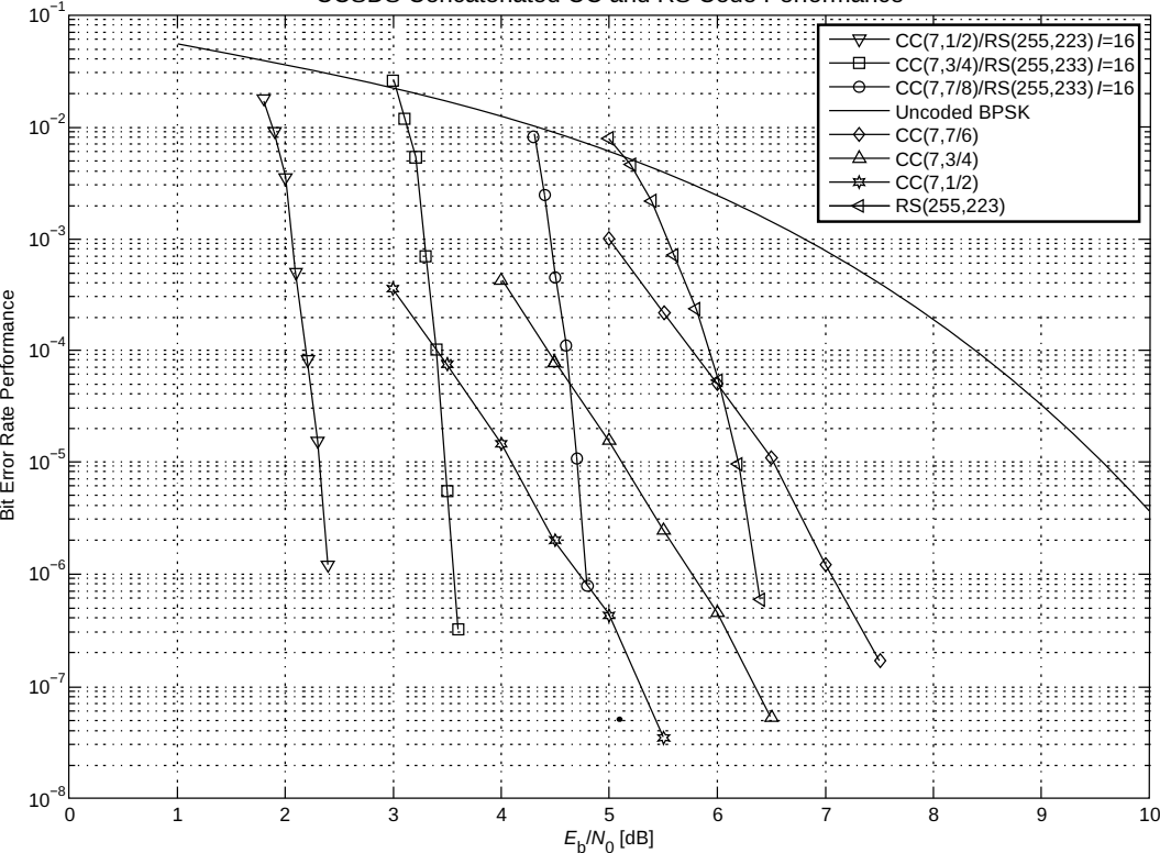
CCSDS Concatenated CC and RS Code Performance
