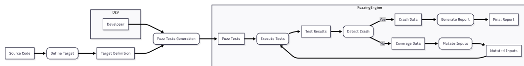
Figure 1.2: The Fuzzing Process. The manual creation of "Fuzz Drivers" (center) is the bottleneck this thesis aims to automate.
