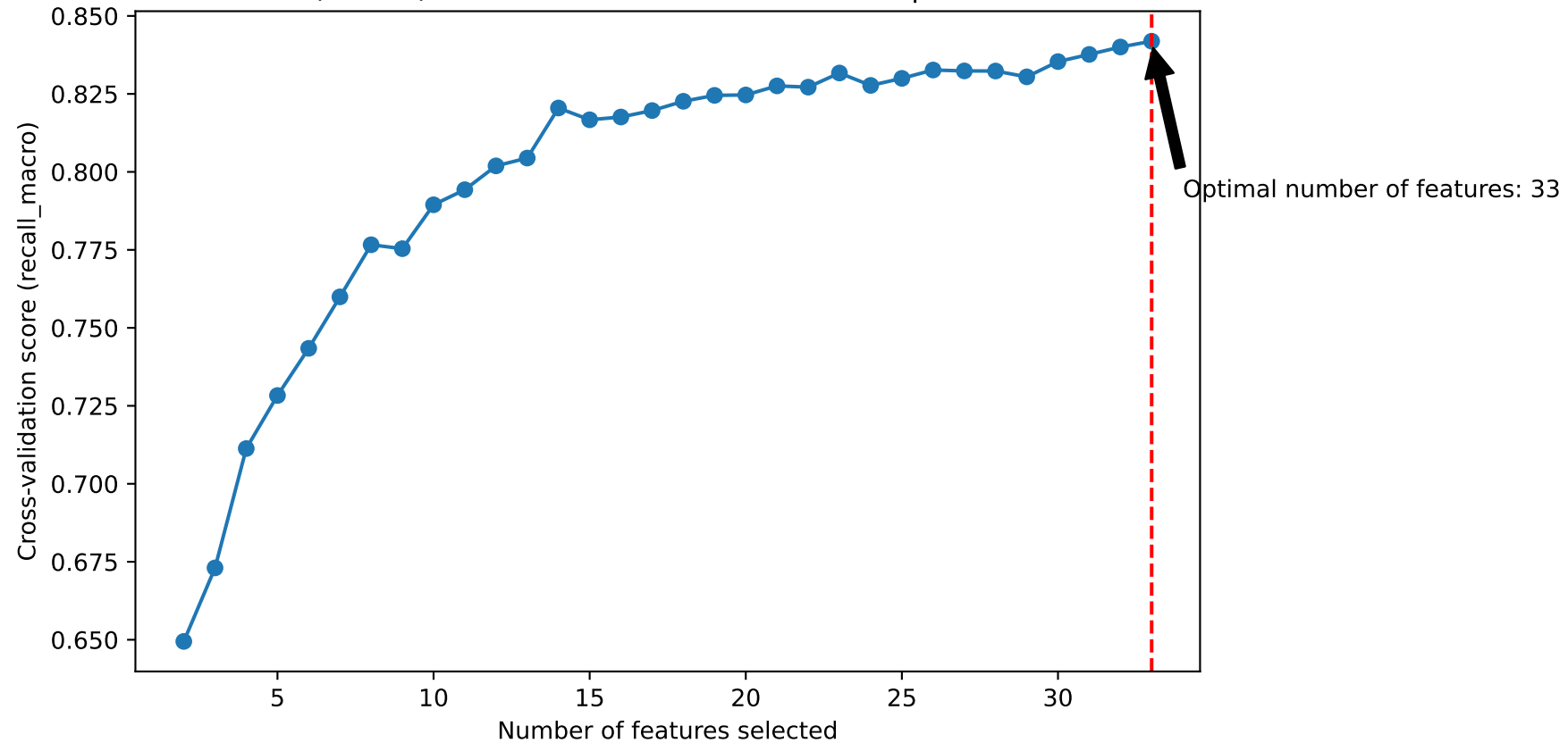
Feature Selection(RFECV) for baseline model - Number of optimal Features selection
