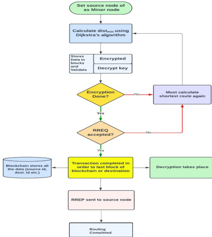
Figure 6.6: Flow process from a route request initiation to the final packet and compute a optimal path.
