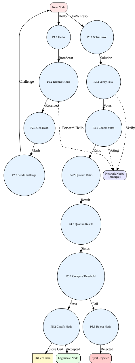
Figure 6.2: Level-2 DFD for Sybil Attack Mitigation
