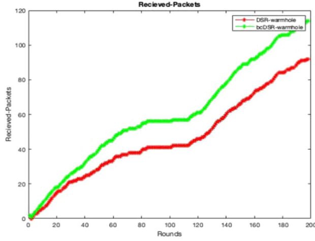
Figure 8.3: More Packets are delivered to host during wormhole occurrence v/s rounds.
