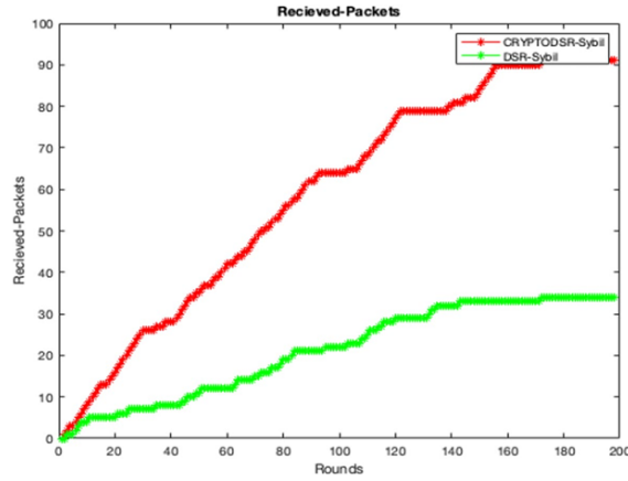
Figure 8.4: Less Packets are delivered during Sybil occurrence as shown in green curve.
