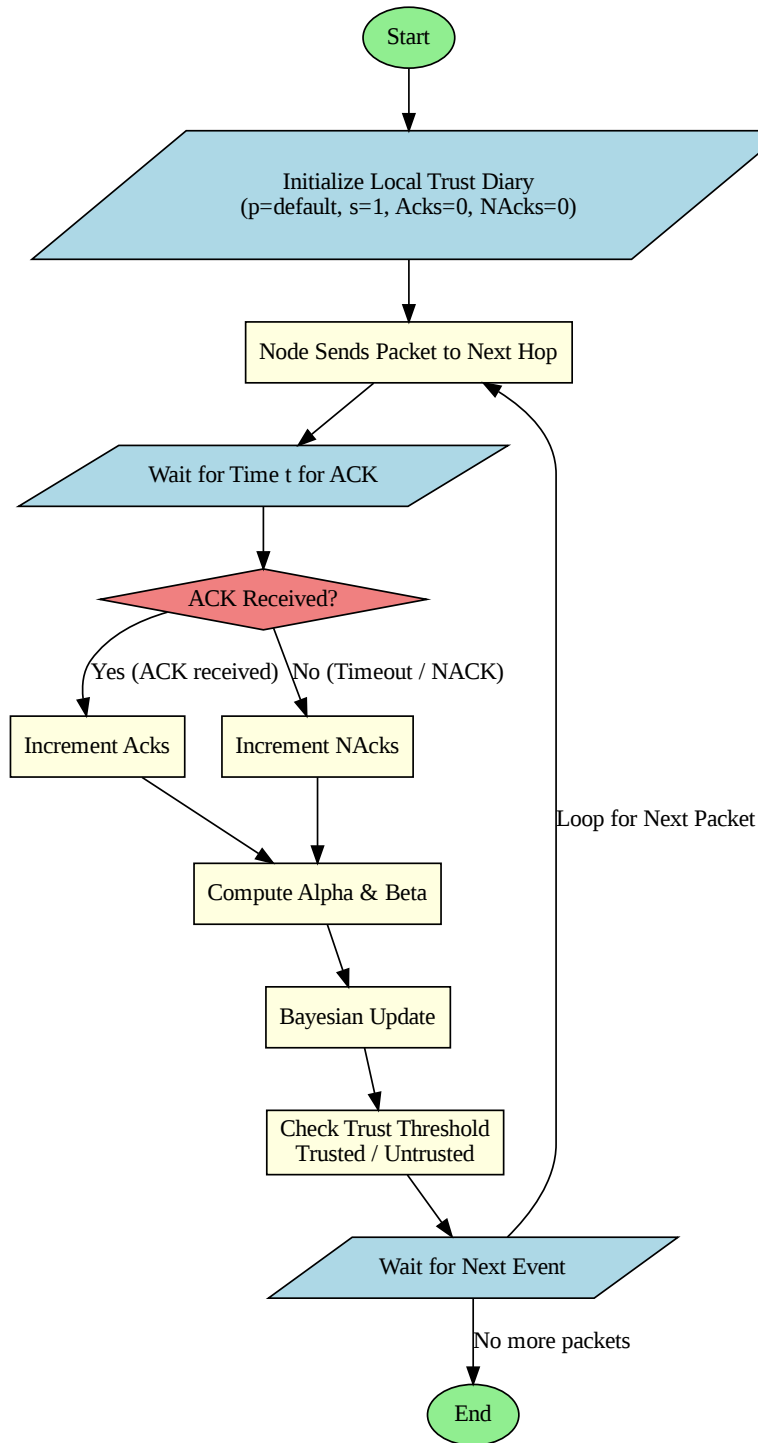
Figure 5.1: Local Trust Diary Flowchart. Trust is represented as a probability distribution and computed on each node.
