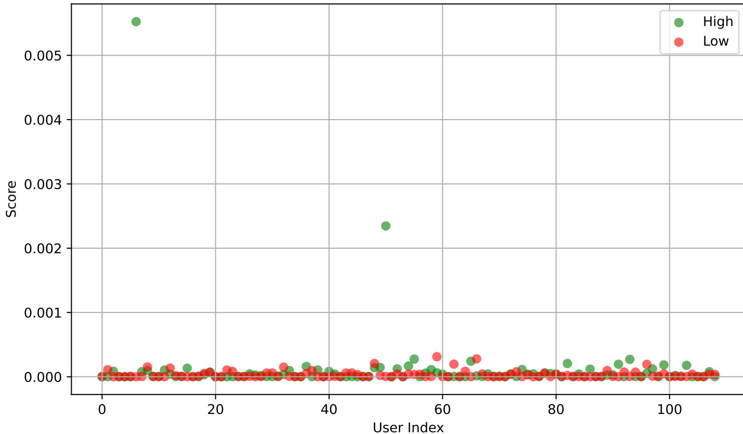
Scatter Plot - AbsoluteTrust
