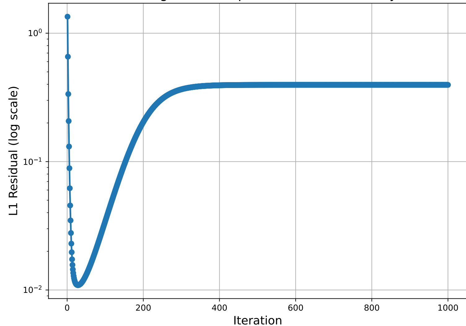
Convergence of RepuLink (Interaction Only)
