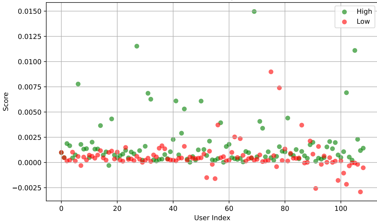
Scatter Plot - PageRank
