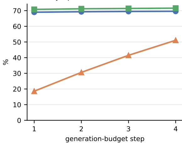
V3: Lab-based Reranking (MRR)
