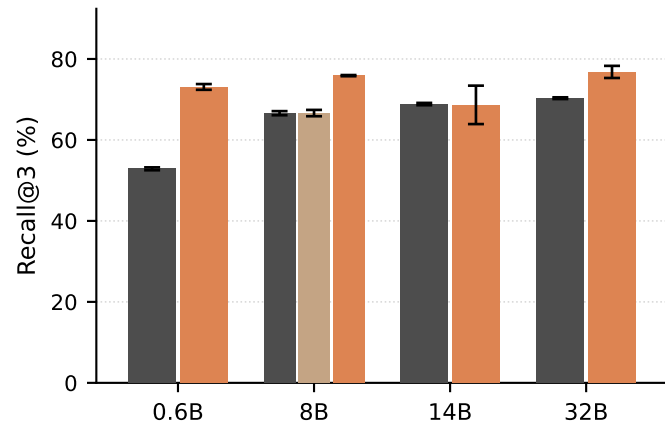
Diagnoses: Recall@3
