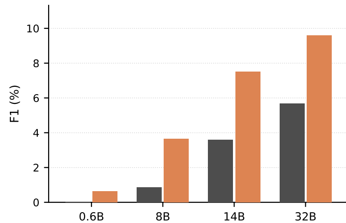
Tail ( < 10 train)
