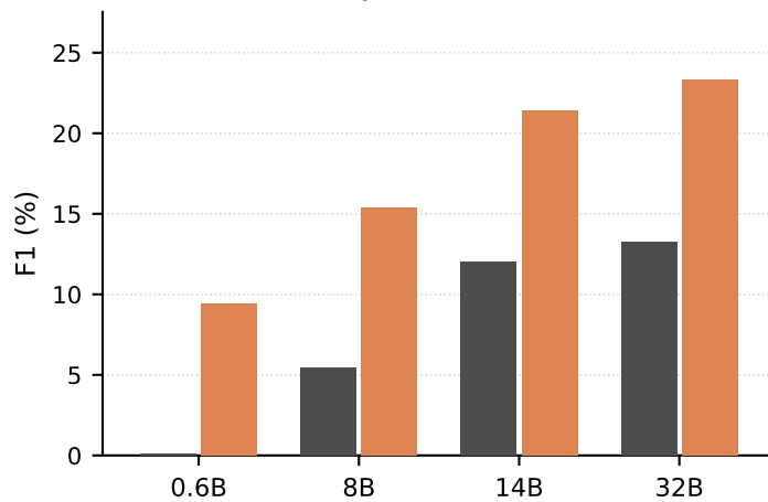
Body (10-99 train)
