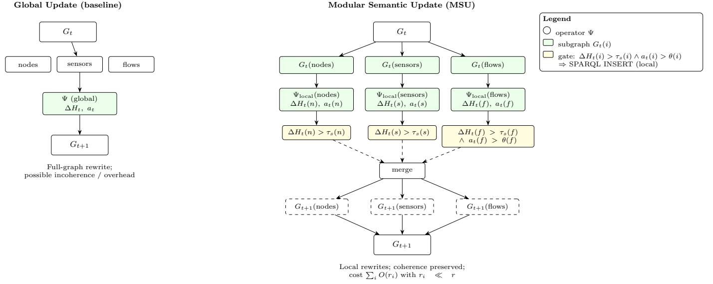
Figure 1: MSU schema: comparison between global update and modular update with \Psi_{\text{local}} on sub-graphs G_t(i) . The thresholds \tau_s(i) and \theta(i) enable conditional updates, reducing overhead and preserving semantic coherence.
