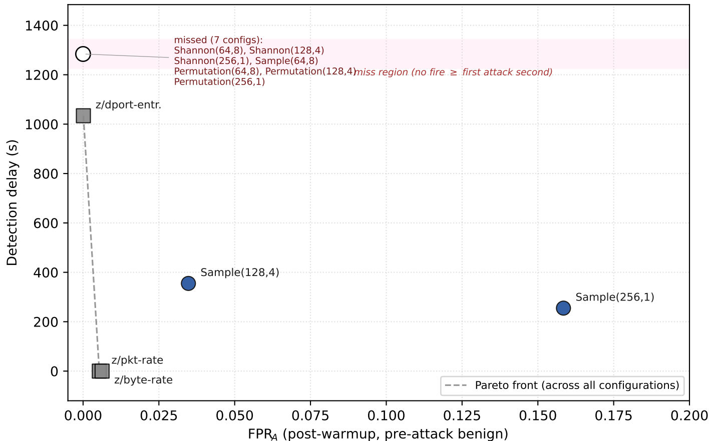
Design-space Pareto front on CIC-IDS2017-aligned proxy stream (circles: EAL configurations; squares: z-score baseline; open circle: missed cluster)
