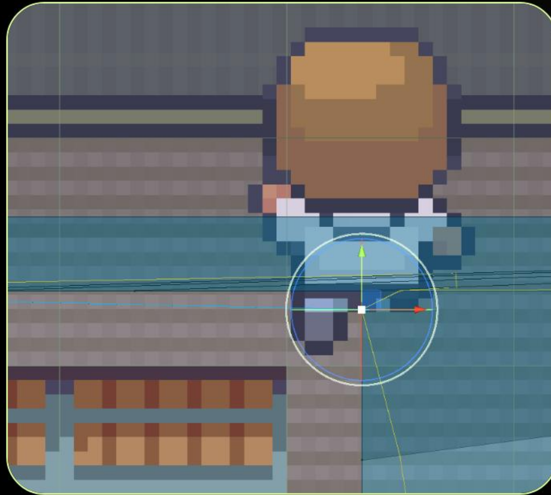
NavMesh Path
