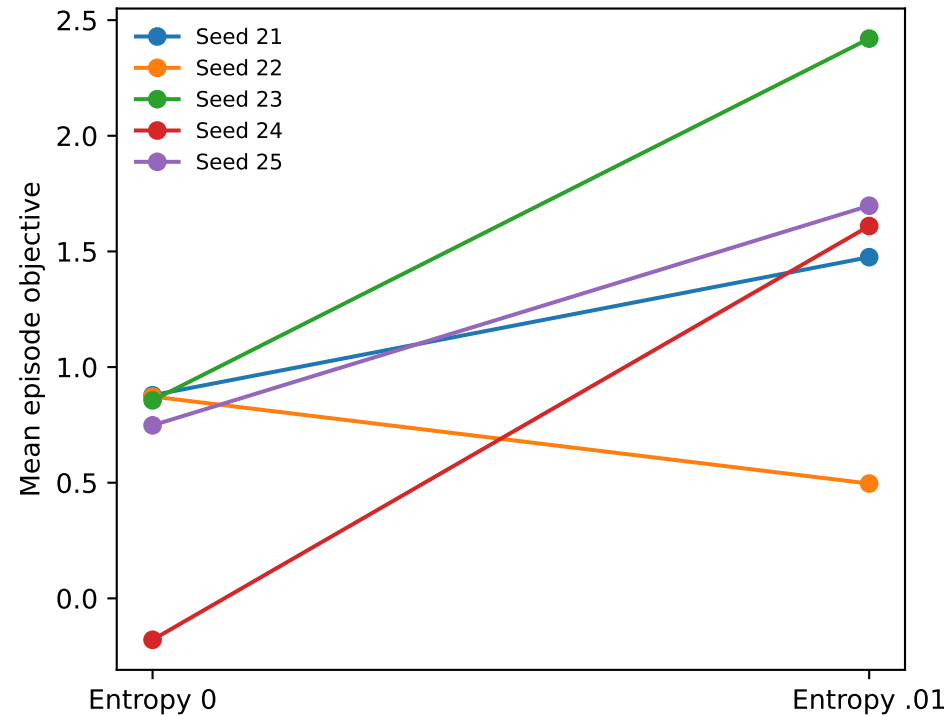
Five independent seed pairs
