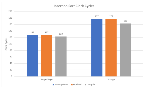
Fig. 9. Clock Cycle Comparison by Algorithm and Processor
