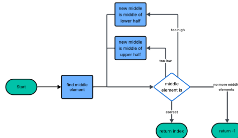
Fig. 3. High-Level Binary Search Flowchart
