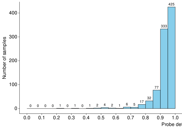
EpicV1
