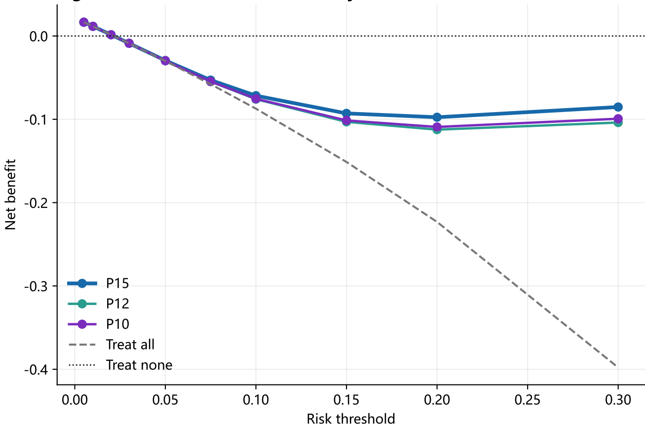
Figure 4. eICU decision curve analysis
