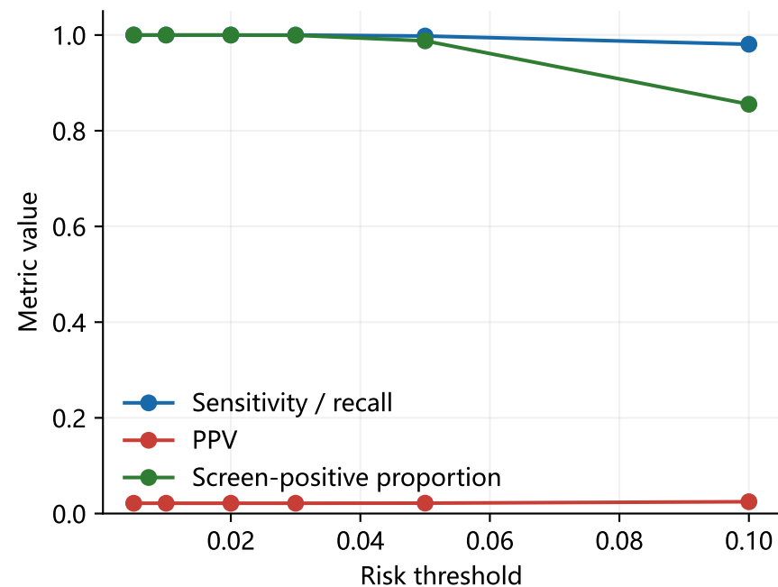
Supplementary Figure S1. P15 threshold-specific operational performance in eICU
