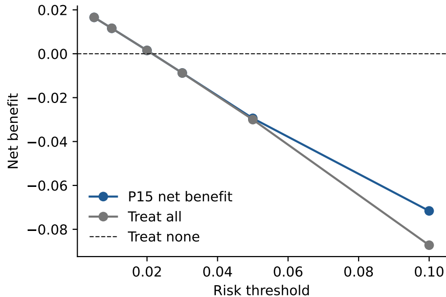
Decision-curve context
