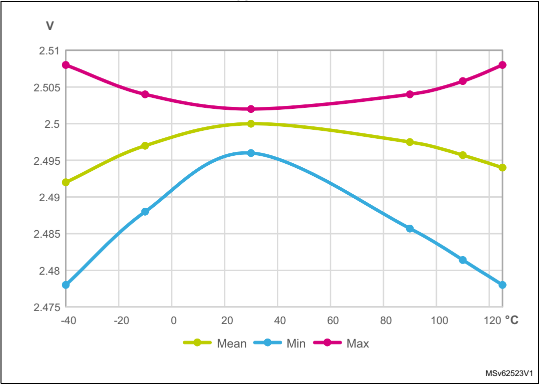
Figure 32. V_{REFOUT} TEMP in case VRS = 01
