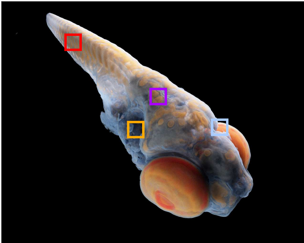
Zebrafish
