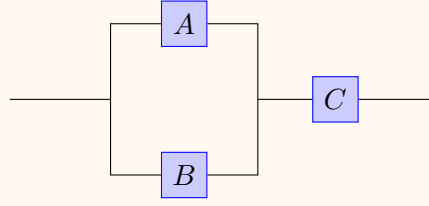
Figuur 1: Circuit diagram with three independent devices.
