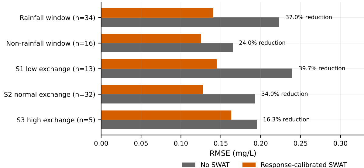
(b) Stratified gains on the test set
