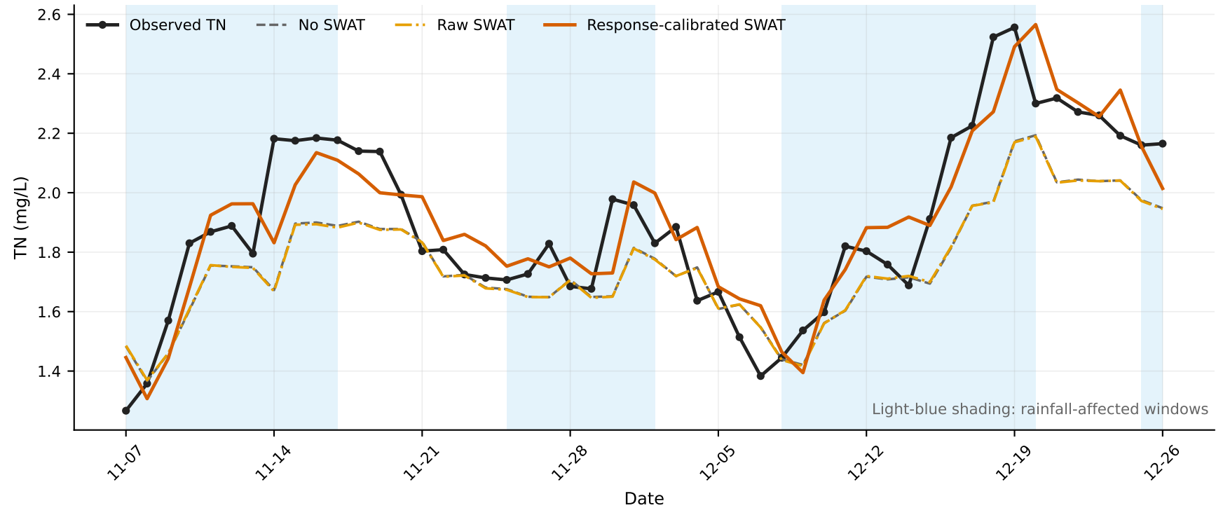
Observed and Predicted TN at the Outlet-Gate Section During the Test Period
