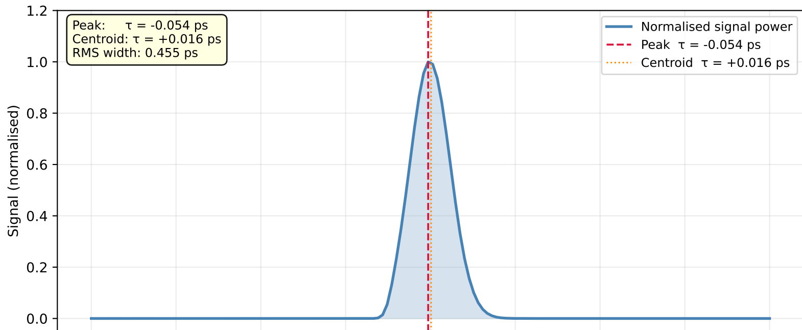
C 2 — Anti-Stokes signal power vs Stokes delay Scenario A — pump 15 cm · Stokes 15 cm
