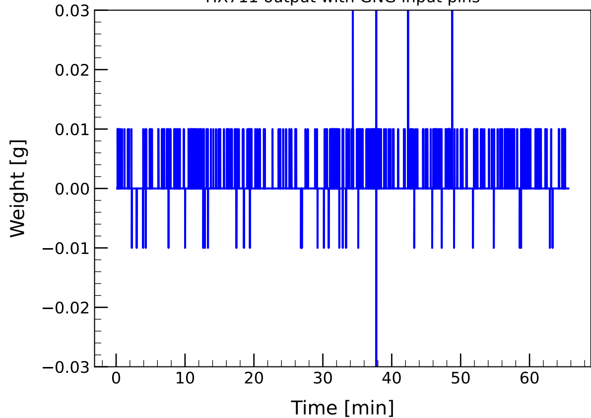
HX711 output with GNG input pins
