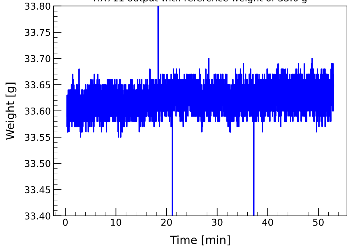
HX711 output with reference weight of 33.6 g
