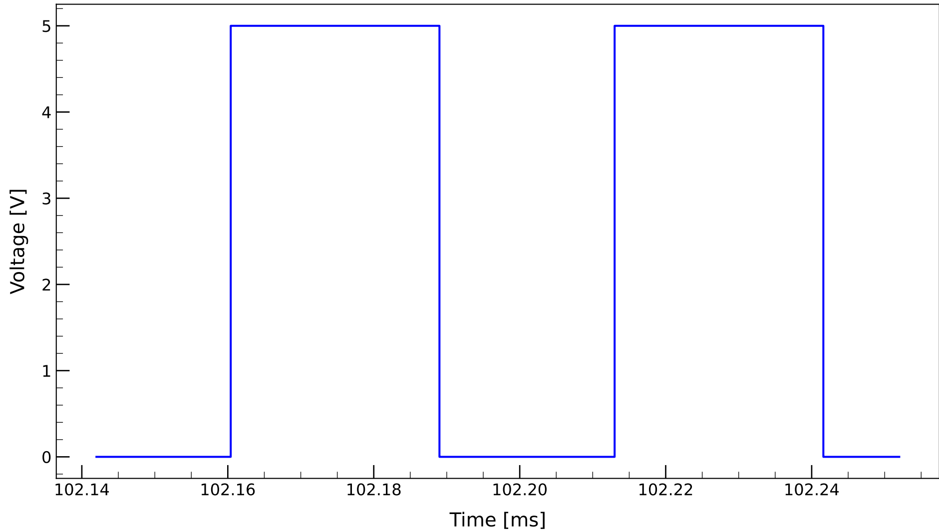
Arduino SCK Signal at HX711 clock input (Zoom)
