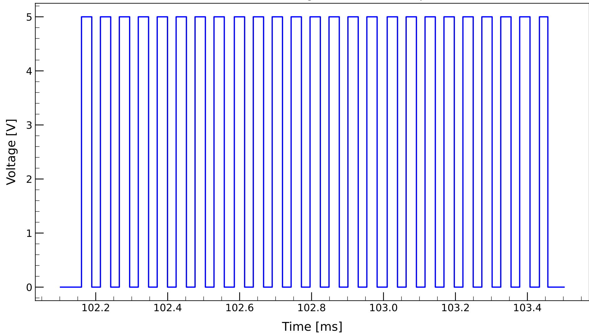
Cleaned Arduino SCK Signal at HX711 clock input
