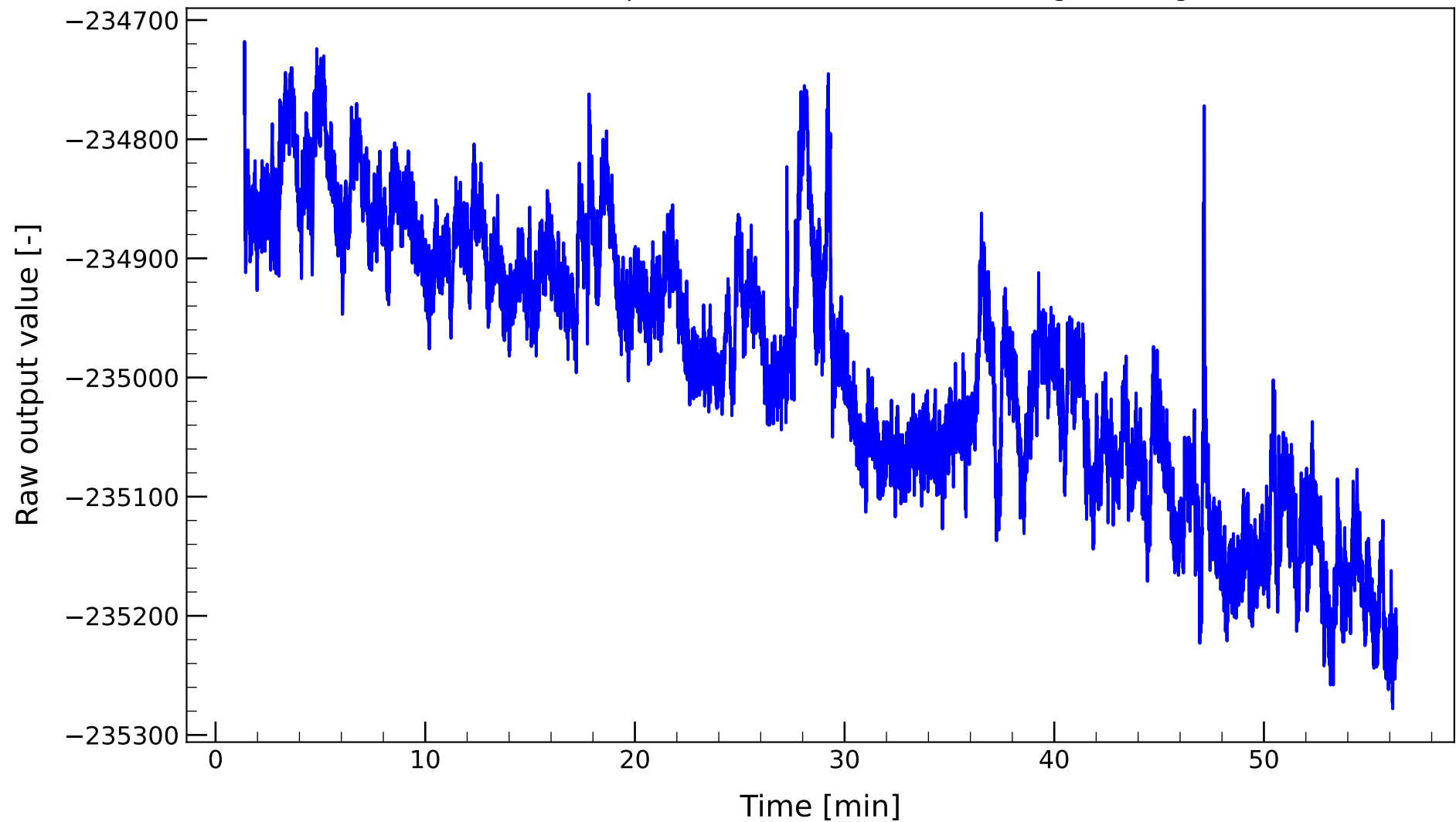
HX711 raw output with FireBeetle with stable weight (33.6 g)
