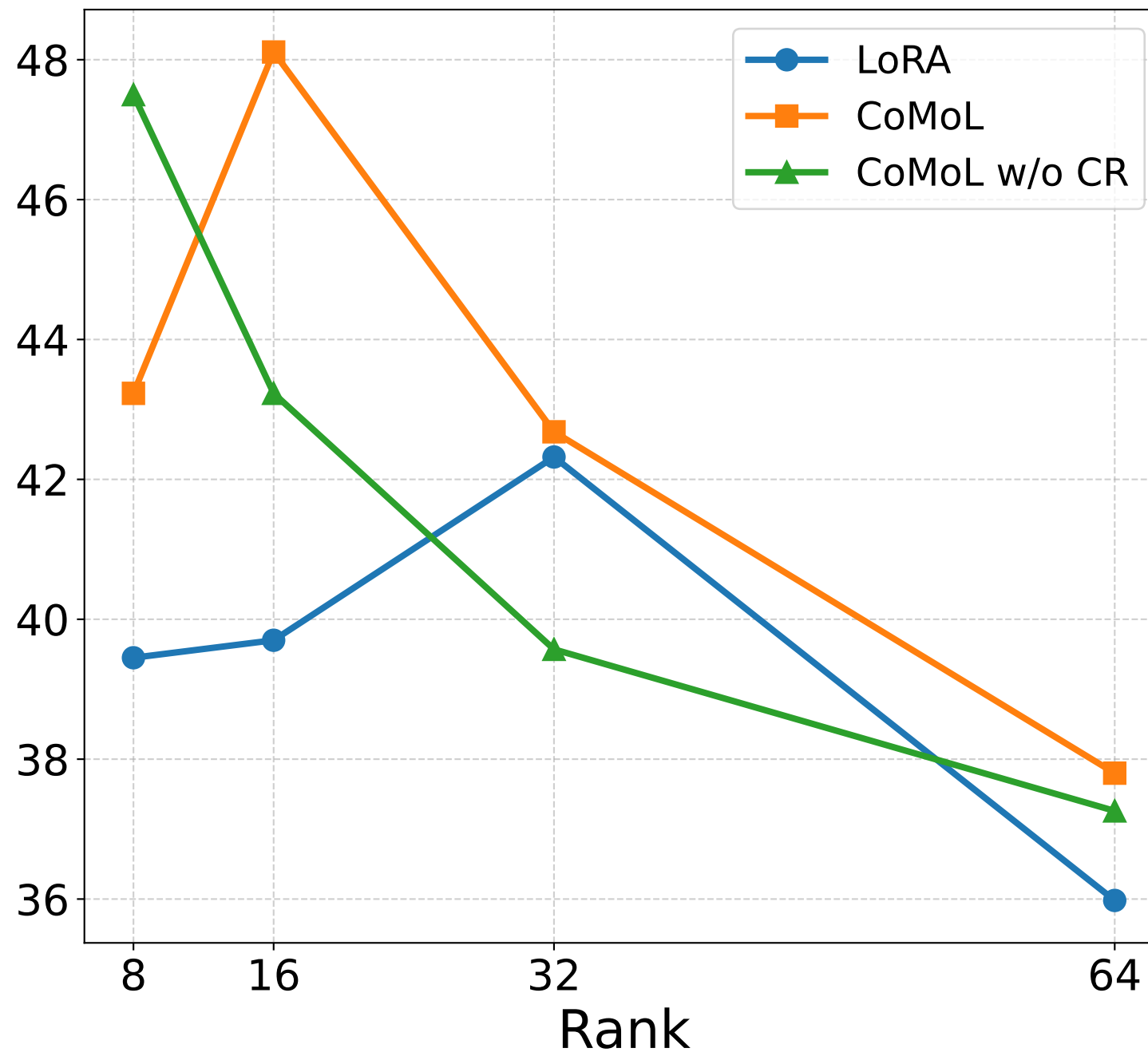
Pass@1 (%)
