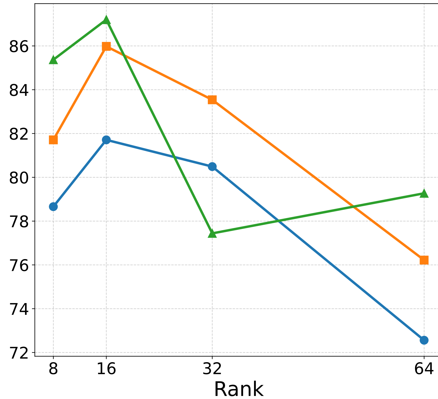
Pass@10 (%)
