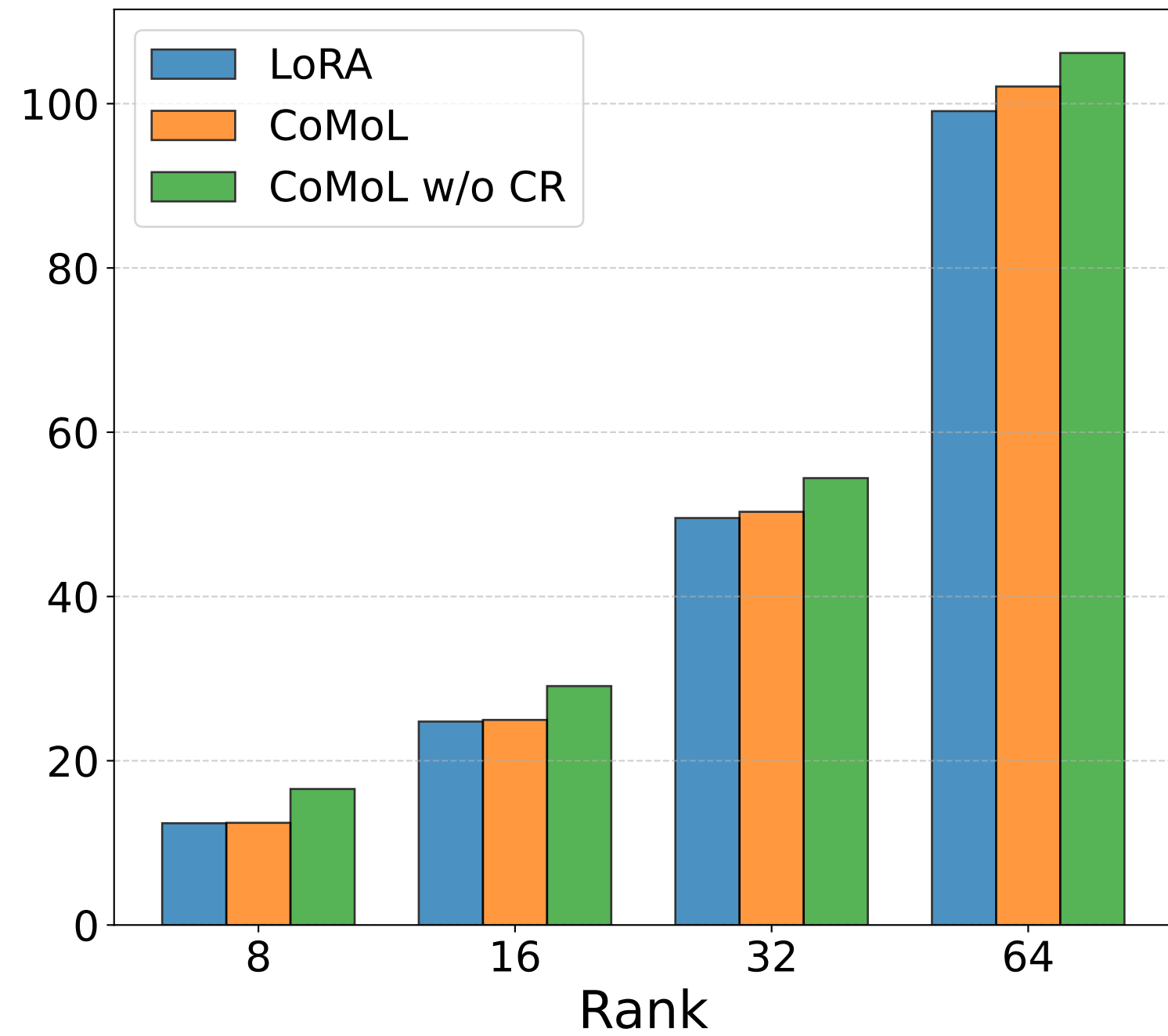
Params (M)
