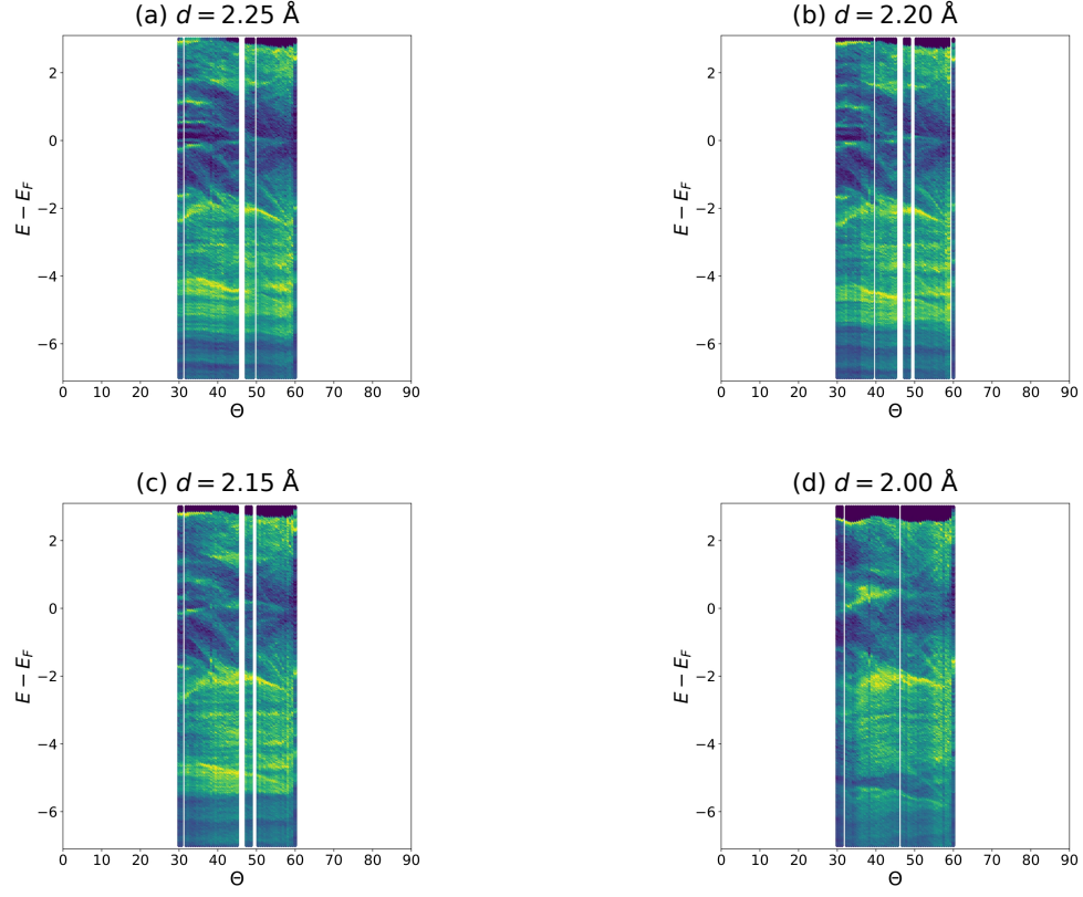
FIG. S3. Original SZV lower-layer projected DOS panels for d = 2.25, 2.20, 2.15 , and 2.00 Å. A missing white column is not a gap. A dark region can reflect small layer weight, broadening, or finite-size discreteness and is not by itself a bulk spectral gap.
