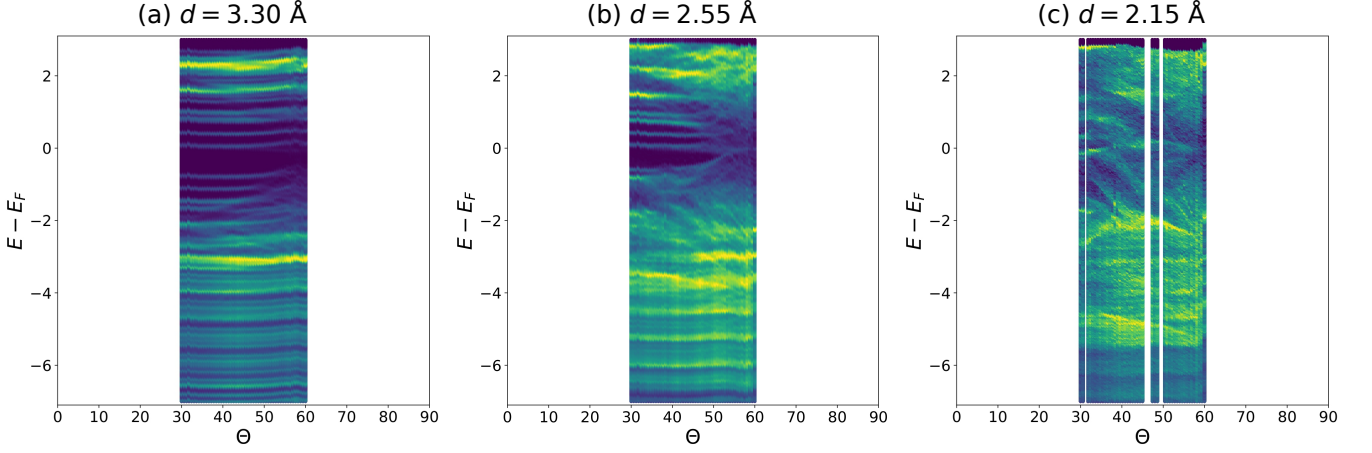
FIG. 2. Evolution of the lower-layer p_z -projected alpha-spin DOS with imposed separation, using SZV-MOLOPT-GTH. The source images are reproduced without intensity manipulation. \Theta is in degrees and E - E_F is in eV. The sampled interval is 30^\circ – 60^\circ . Dark-to-bright colors encode increasing weight, normalized separately to each column's maximum. White columns indicate unavailable data in the original plotting workflow. The finite printed-state window limits interpretation at positive energies (SM). All ten distances and the DZVP comparisons are shown in the SM.
