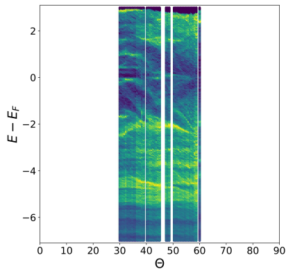
(b) SZV, d = 2.20 Å
