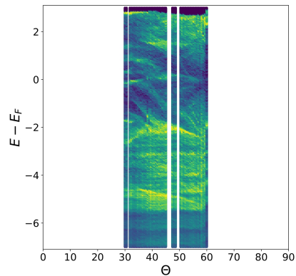
(c) SZV, d = 2.15 Å
