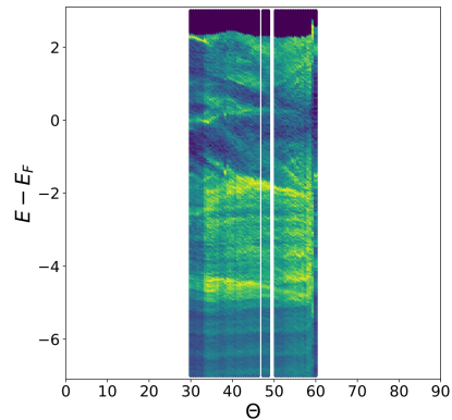
(f) DZVP, d = 2.15 Å
