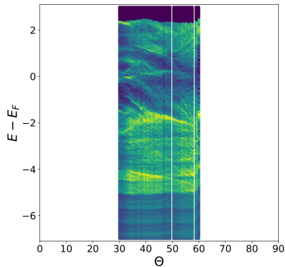
(e) DZVP, d = 2.20 Å
