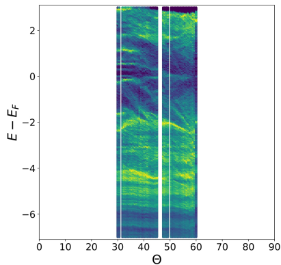
(a) SZV, d = 2.25 Å
