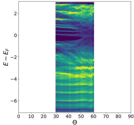
(b) d = 2.55 \text{ \AA}
