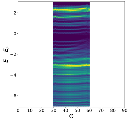
(a) d = 3.30 \text{ \AA}
