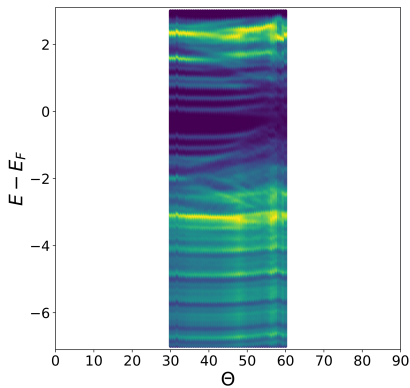
(b) d = 3.00 \text{ \AA}
