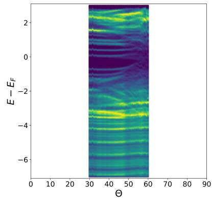
(c) d = 2.85 \text{ \AA}
