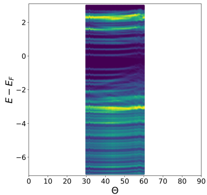
(a) d = 3.30 \text{ \AA}
