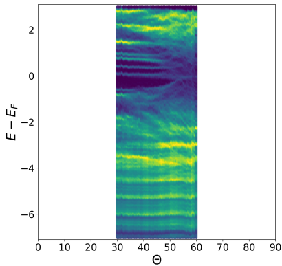
(e) d = 2.55 \text{ \AA}
