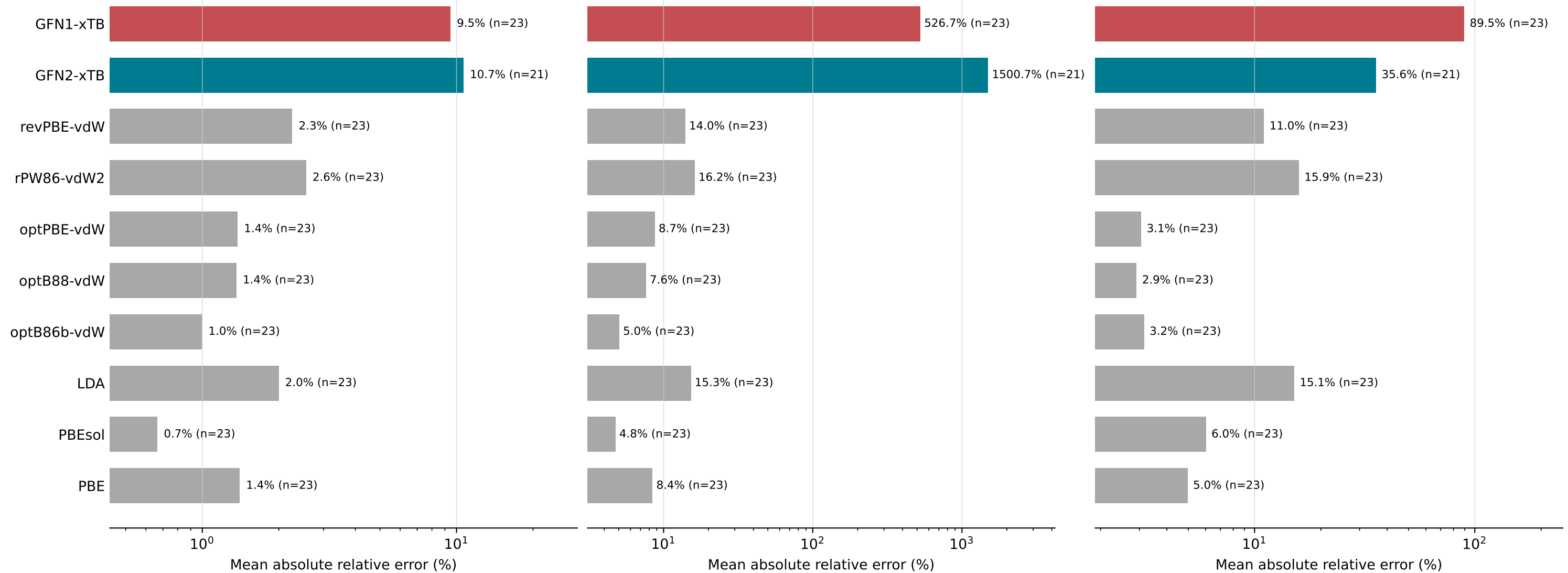
Lattice constant
