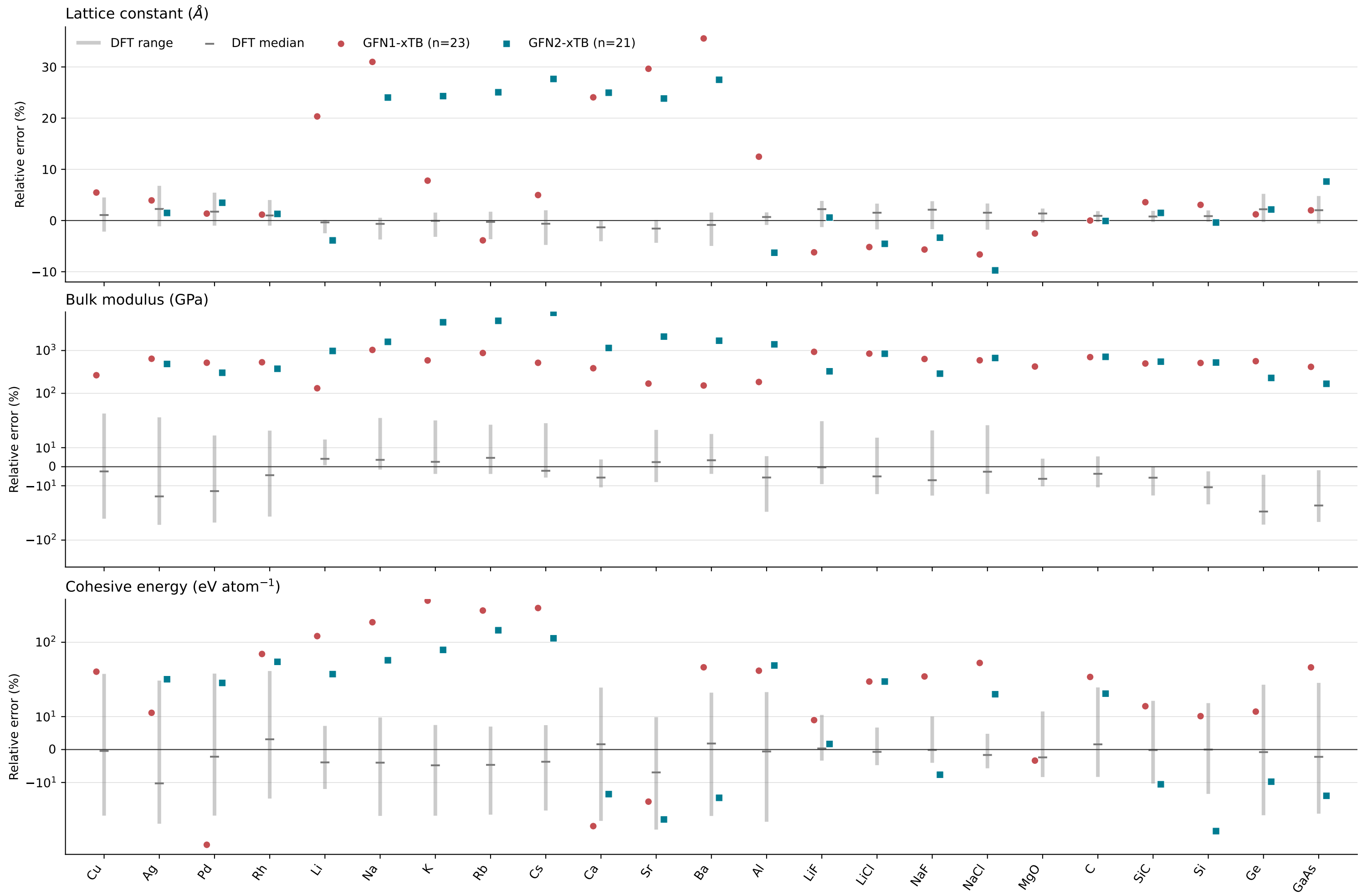
Klimes-23: system-wise errors against experiment
