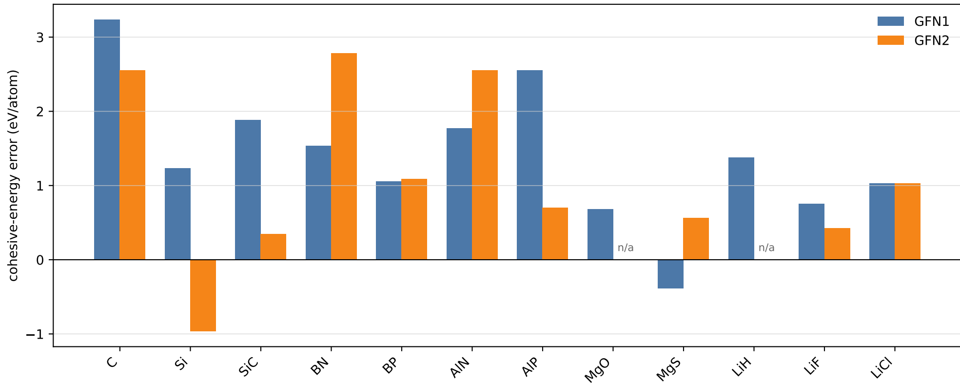
LC12 (Goldzak12) EOS CP2K/tblite native-Bloch k555
