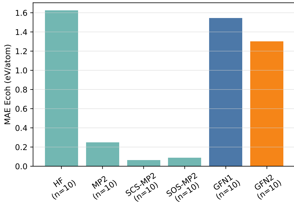
LC10 comparison to zero-point corrected experiment
