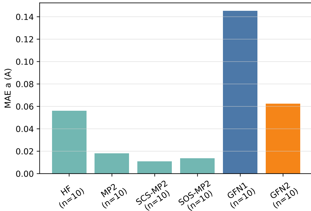
LC10 comparison to zero-point corrected experiment
