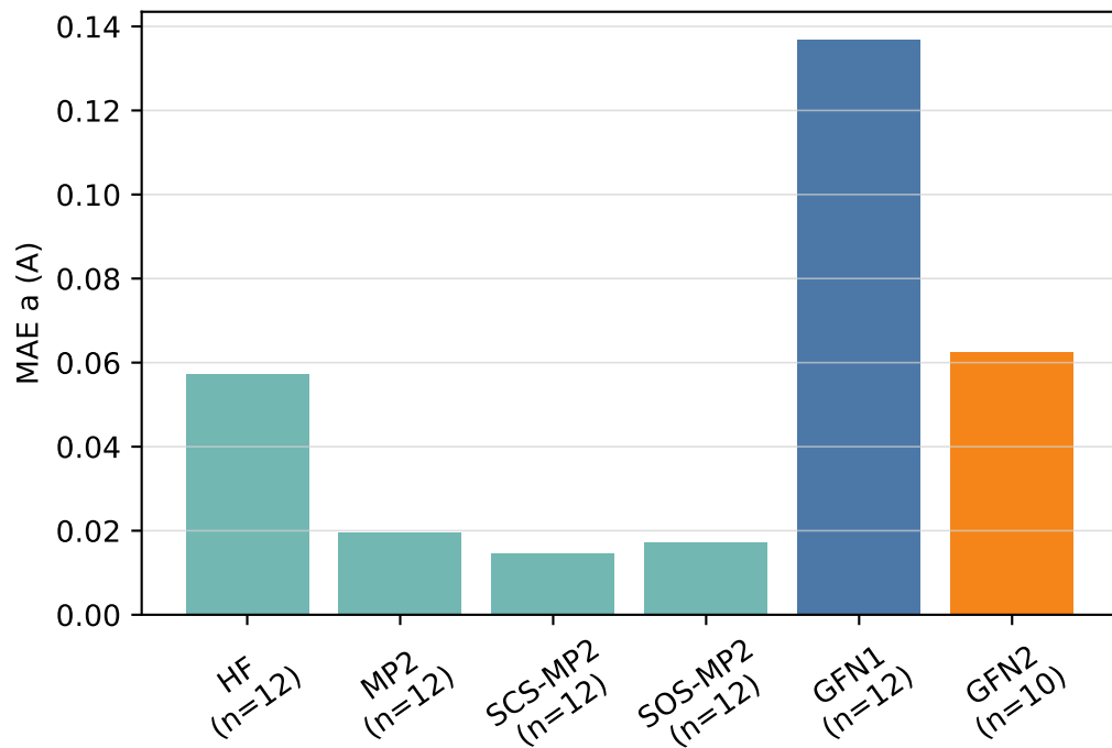
LC12 (Goldzak12) comparison to zero-point corrected experiment
