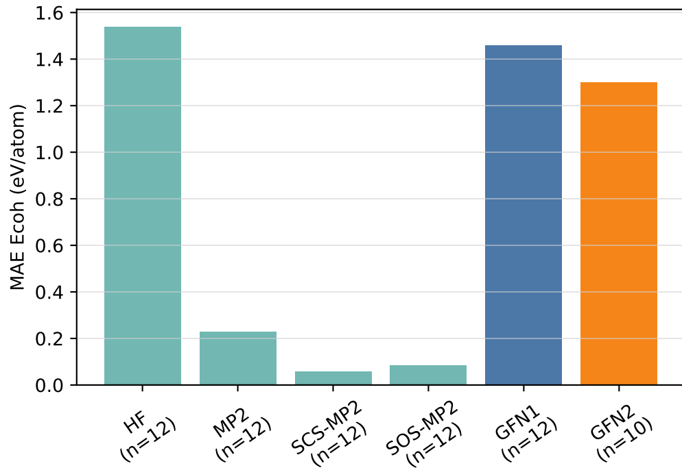
LC12 (Goldzak12) comparison to zero-point corrected experiment
