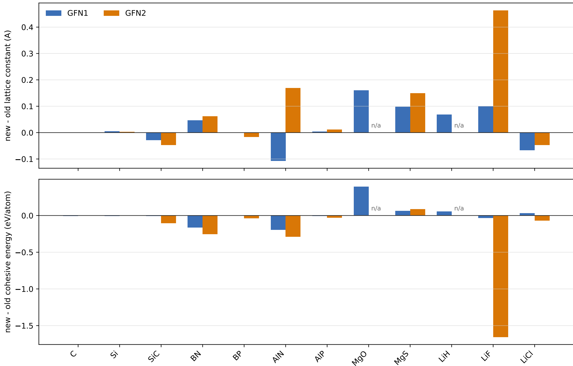
LC12 current stack versus previous results (k555 native Bloch)
