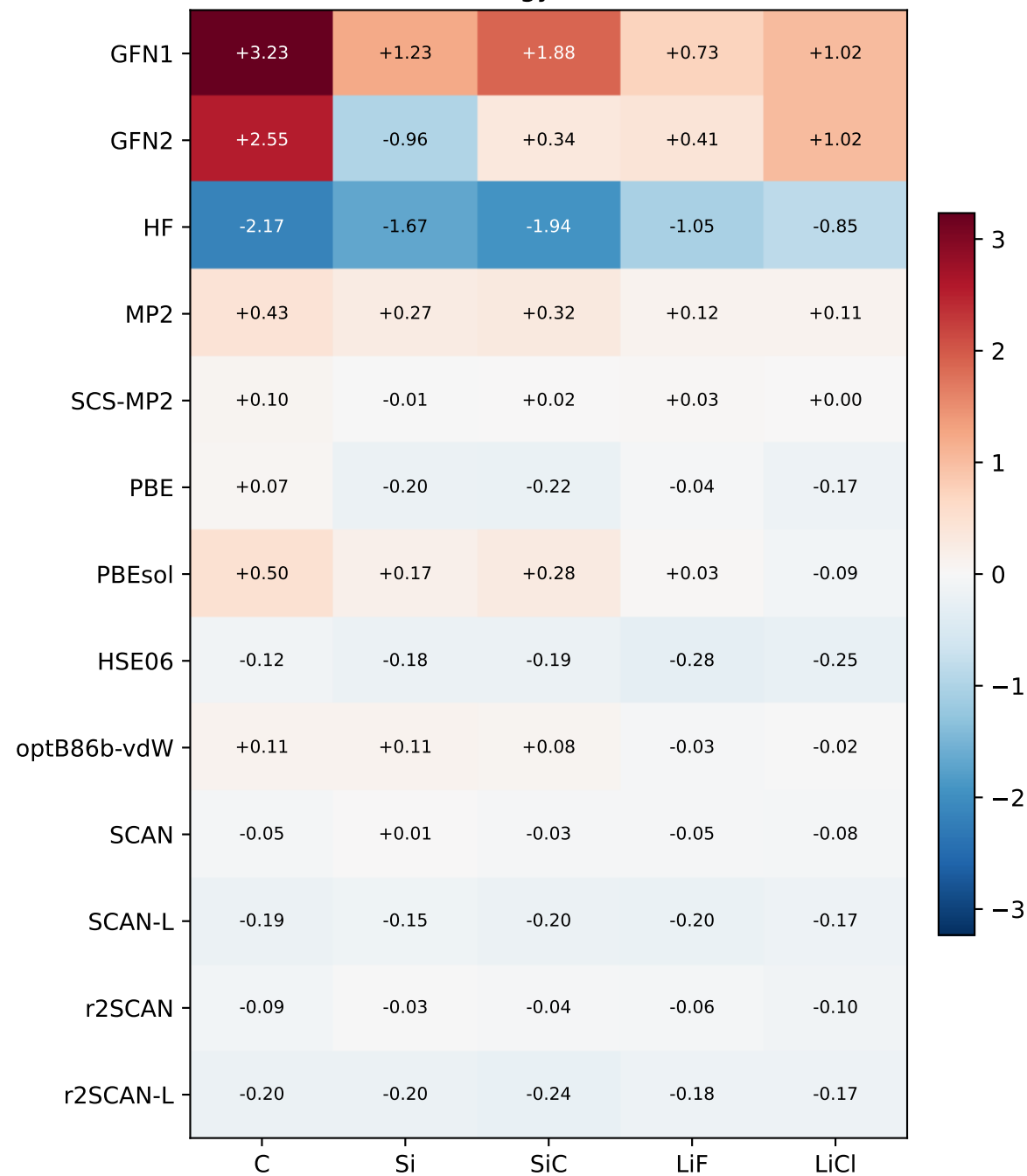
Cohesive-energy error (eV/atom)
