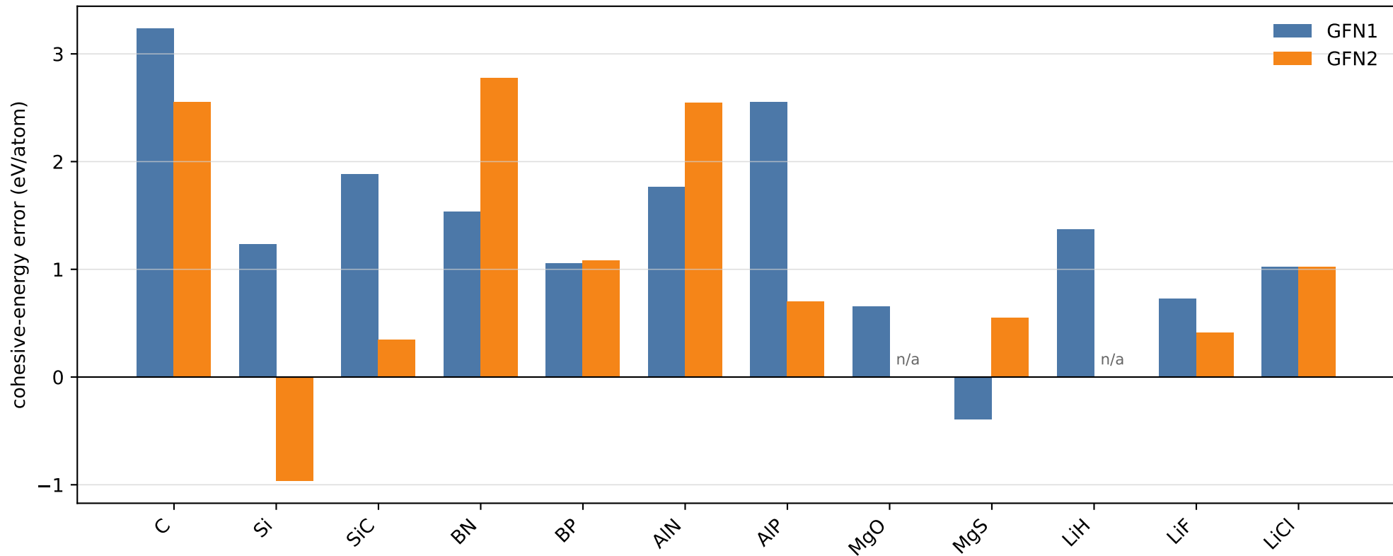
LC12 (Goldzak12) EOS CP2K/tblite native-Bloch k444
